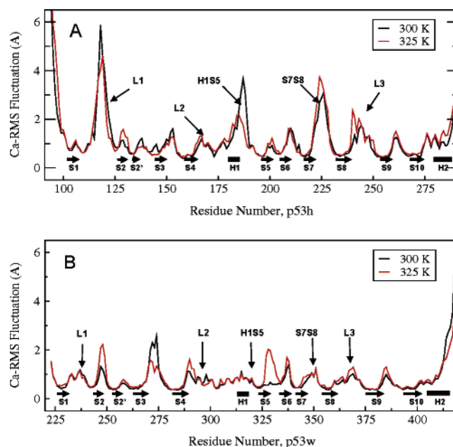
FIGURE 3: Residue-based C \alpha atom root-mean-square fluctuations for the human p53 (p53h) and the worm p53 (p53w) derived from the simulations in Figure 2. This figure allows the direct comparison of fluctuations for specific regions from the human and worm form proteins. Locations of the secondary structures are labeled with horizontal arrows for \beta -strands and rectangular bars for \alpha -helices. Regions with the most dramatic contrast in fluctuation between p53h and p53w are indicated with thin arrows.
