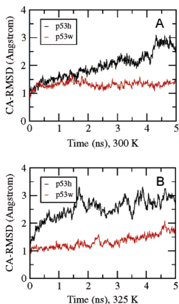
FIGURE 2: C \alpha atom root-mean-square deviations (RMSD) derived from simulations at 300 and 325 K from both the human p53 (p53h) and worm p53 (p53w) core domain from their crystal structures, respectively. The plots show that p53h is very unstable at both temperatures while p53w was stable even at elevated temperature. The three terminal residues at both the N- and C-termini were excluded in the calculations.
