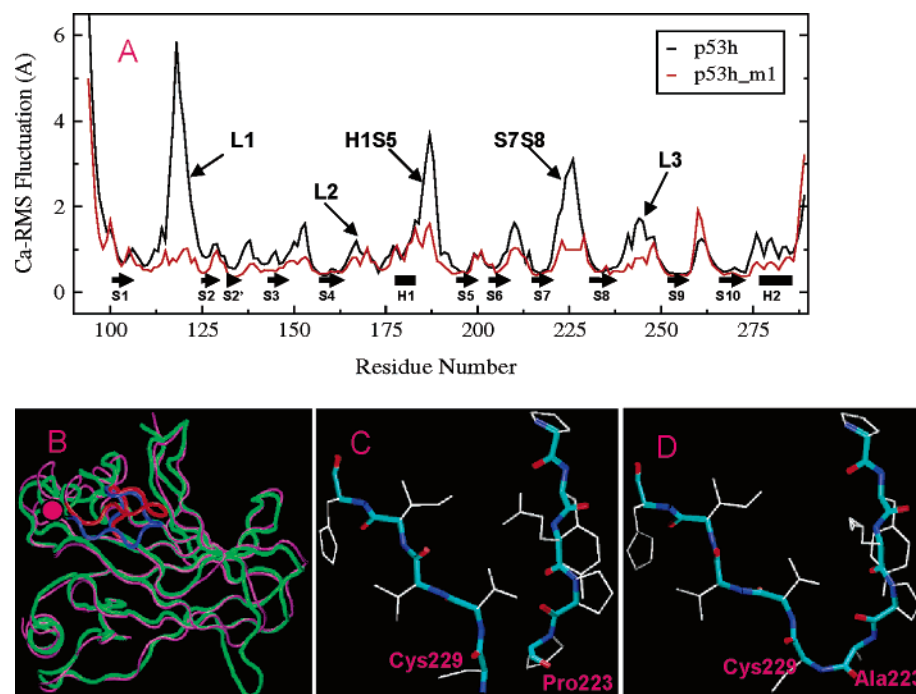
FIGURE 7: Structural properties of the S7S8 turn mutant in comparison with the wild type. (A) Residue-based C \alpha RMS fluctuations for the wild type and the S7S8 turn mutant of the human p53 derived from the 5 ns simulations. Secondary structures were labeled the same way as in Figure 3. The data here show a great impact of the mutation on the overall stability of the protein, with the flexibility reduced in most mobile regions, including loop L1 and turn H1S5. (B) The backbone trace of the mutant structure averaged over the 5 ns trajectory superimposed on that of the wild-type crystal structure. (C) The atomic detail conformation of the turn S7S8 region in the wild-type crystal structure. The five residues at the center of the turn were not shown. (D) The atomic detail conformation of the turn S7S8 region in the mutant average structure. This result shows that, upon mutation, the stability of the protein was greatly increased and the native conformation was well retained by the mutation.
